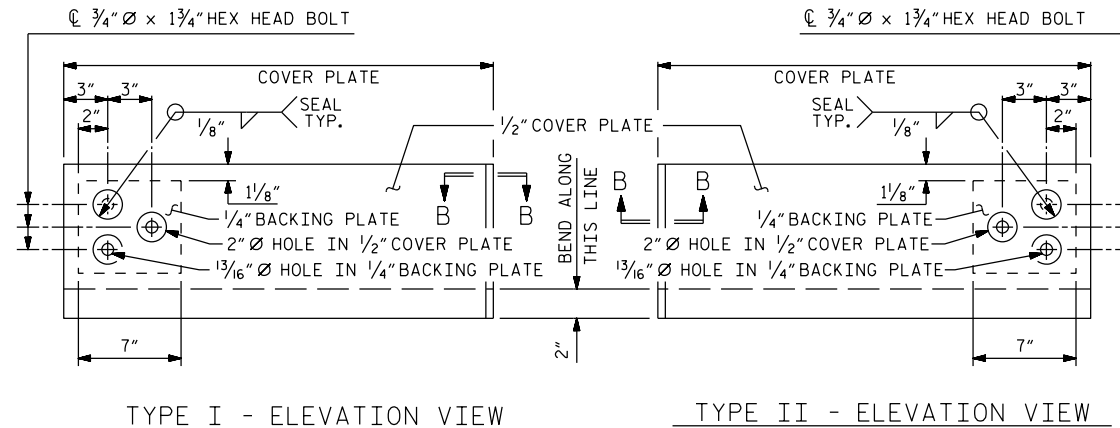
TYPE I - ELEVATION VIEW
